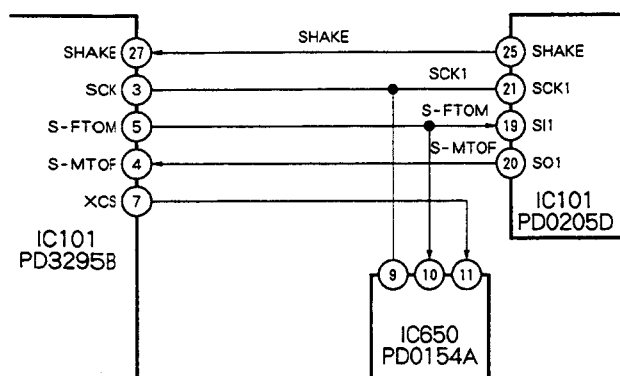
Fig. 2 Serial interface connection diagram
