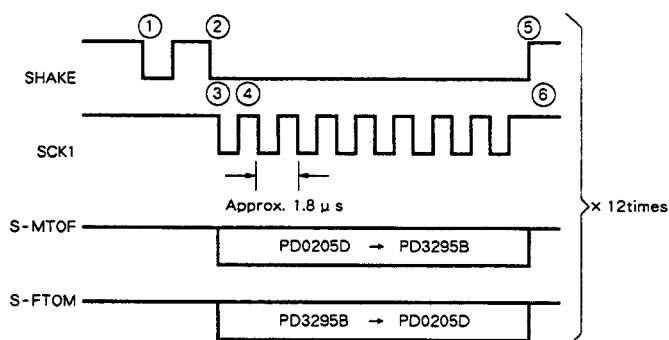
Fig. 3 Timing chart of the microcomputer interface
