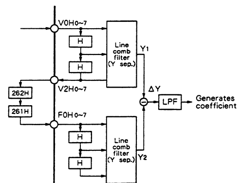
Fig. 6 Y difference detection circuit
