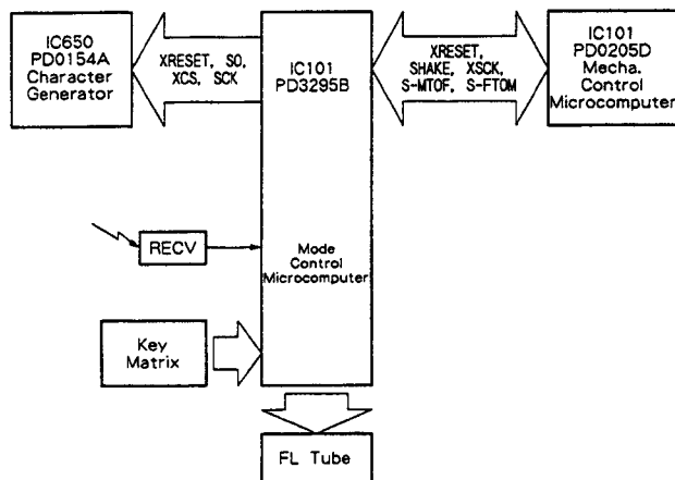
Fig. 1 Mode control block diagram
